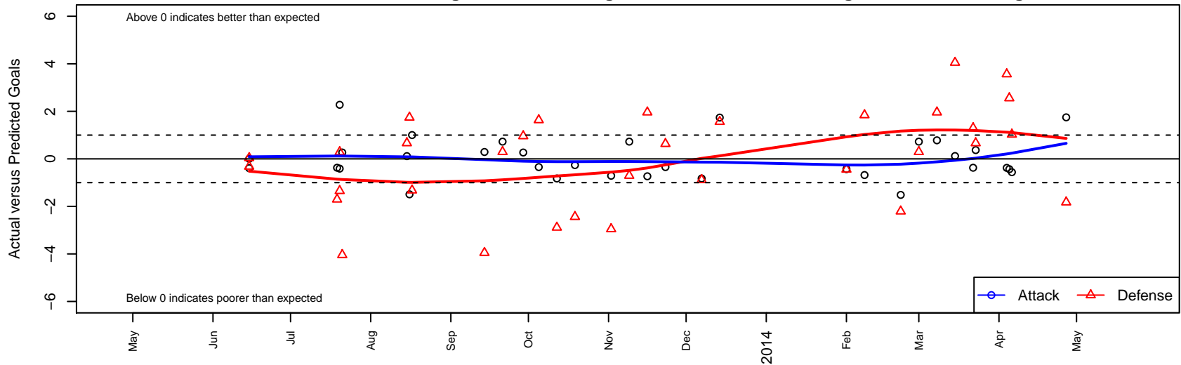
WPFC Fury Black G02 Dots are actual minus expected GF (blue circles) and GA (red triangles). Blue line is smoothed change in attack strength. Red is smoothed change in defense strength.
